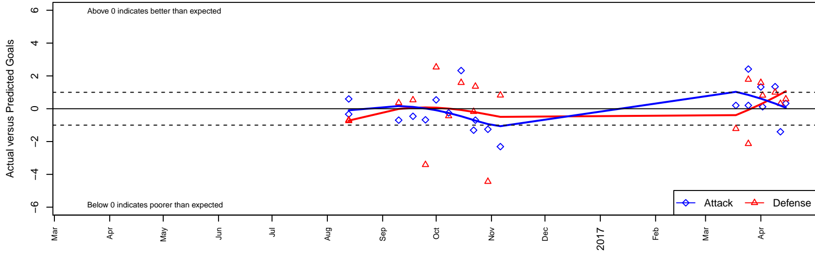
Wenatchee Valley United Barboza G03 Dots are actual minus expected GF (blue circles) and GA (red triangles). Blue line is smoothed change in attack strength. Red is smoothed change in defense strength.
